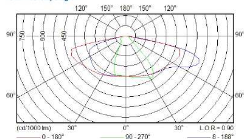
Polar intensity diagram
